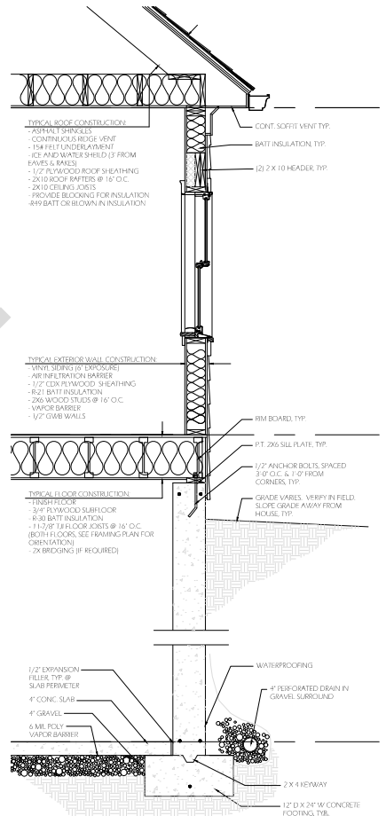
3 DETAILED WALL SECTION SCALE: 3/4" = 1'-0"
