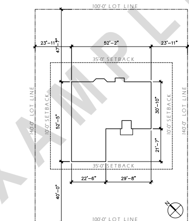
4 PLOT PLAN SCALE: 1" = 20'-0"
